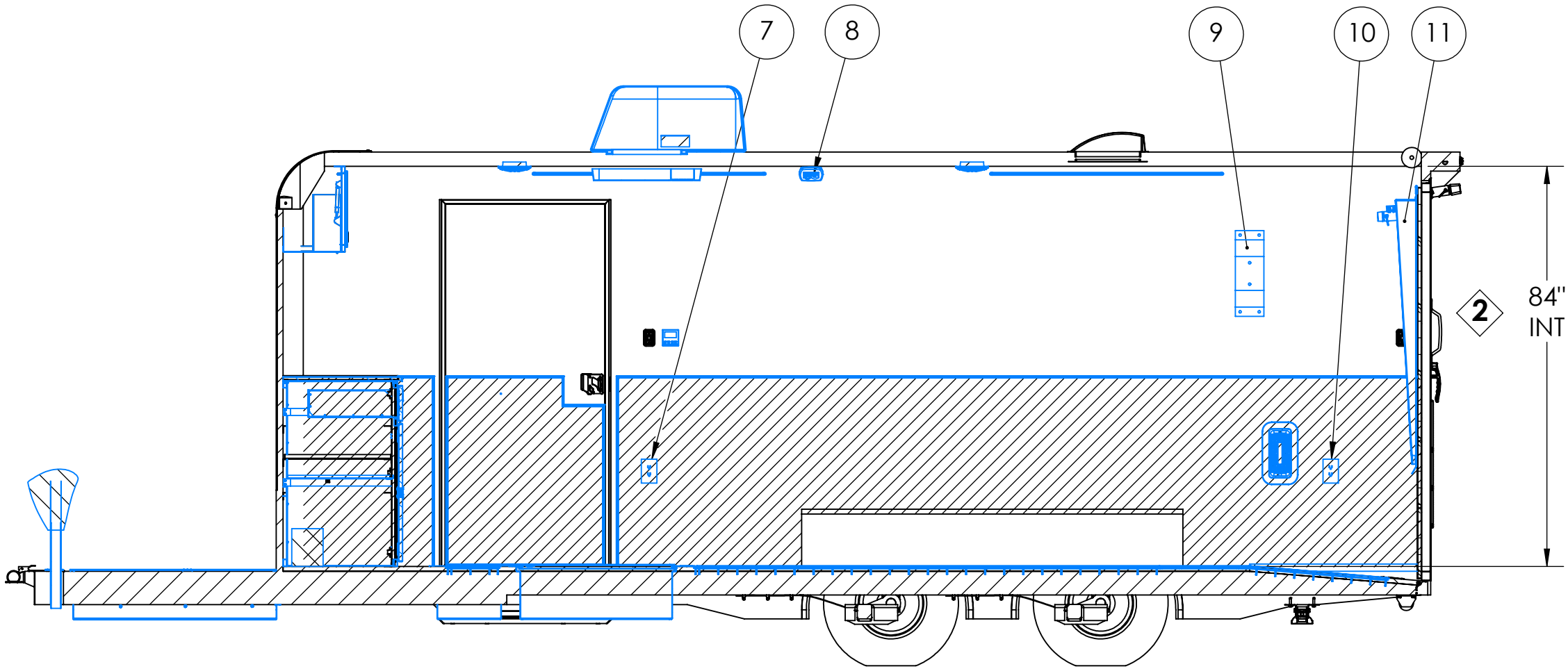
SECTION C-C SCALE 1 : 28
